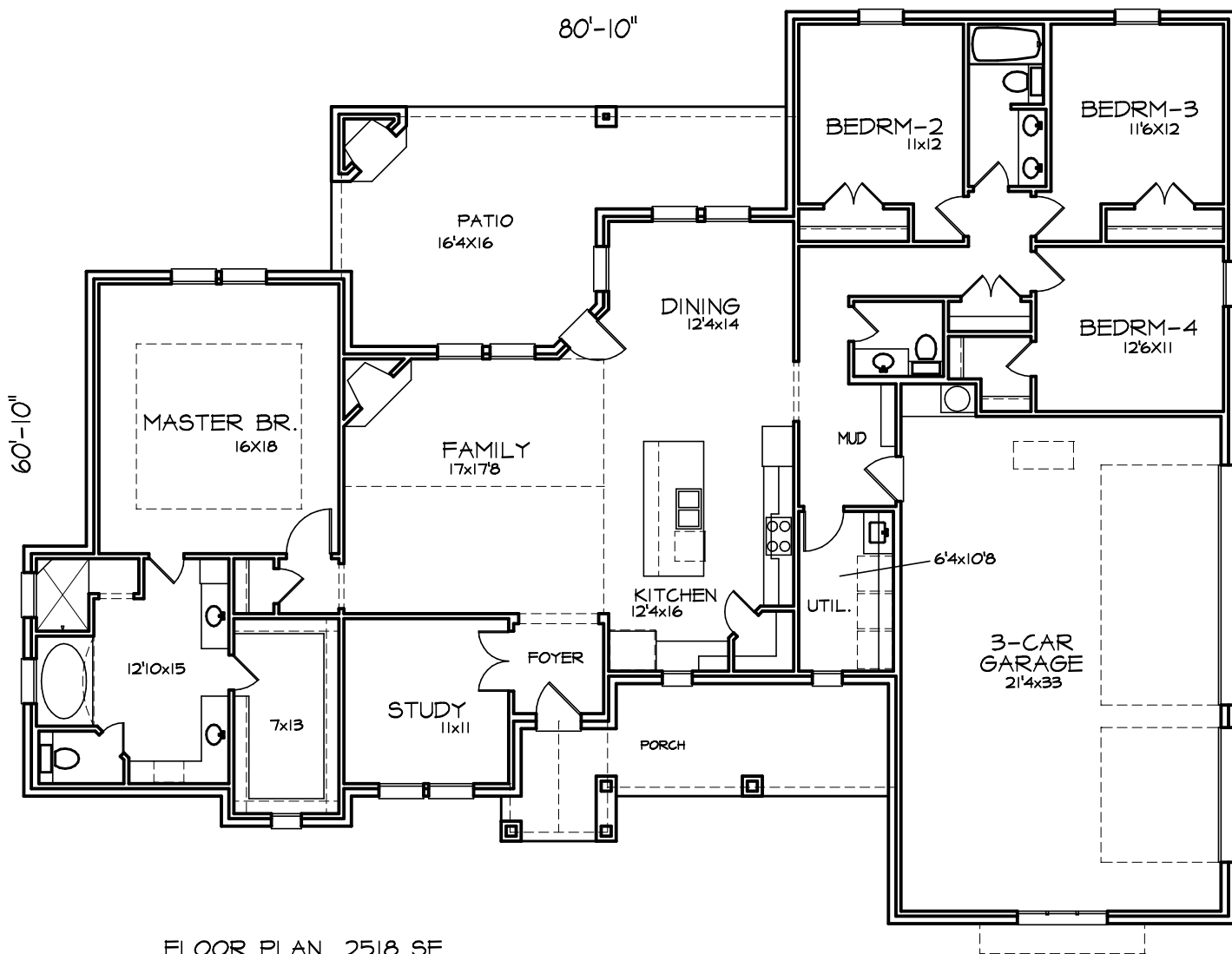
FLOOR PLAN 2518 SF
